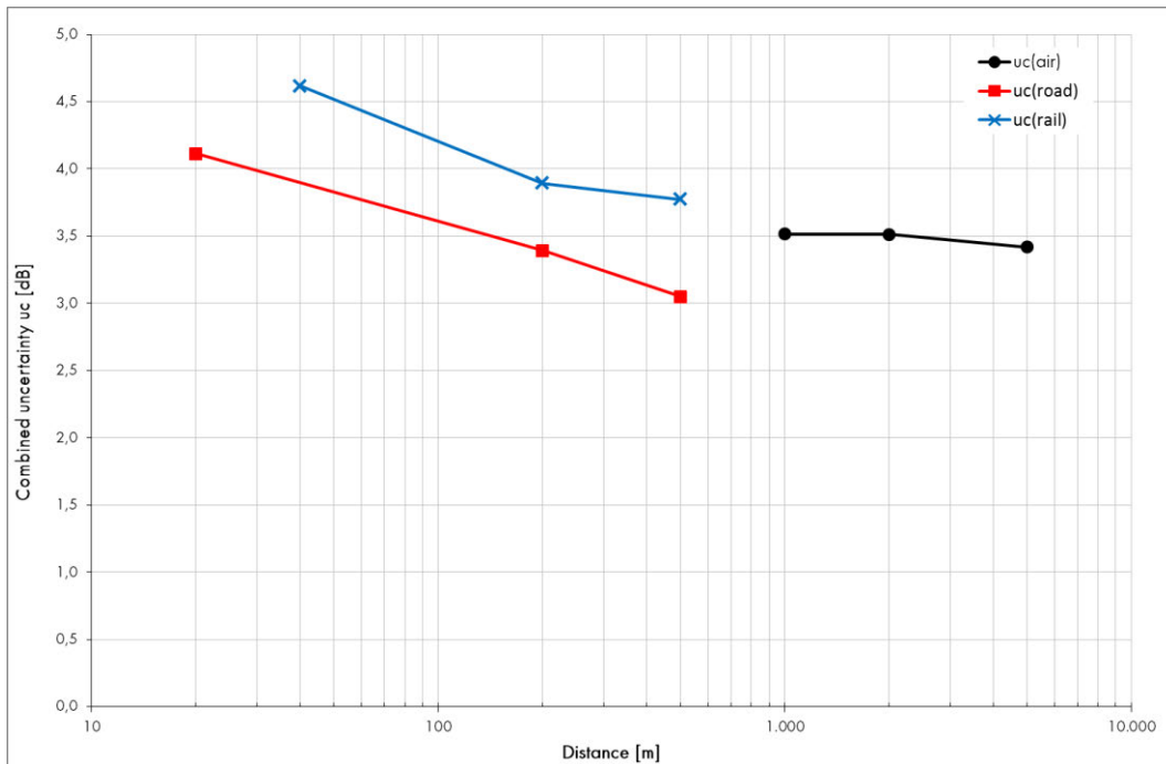
Figure 1: Combined standard uncertainty u_c for air, road and rail traffic noise depending on distance
